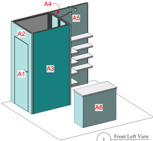
1 Front Left View Scale: 1:60
